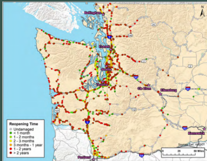
Bridge Seismic Screening Tool (BSST) Projected Reopening Times of Highway Bridges in Washington after the Cascadia Subduction Zone Scenario Earthquake Graphic Courtesy of Washington State Transportation Systems RRAP, March 2019
